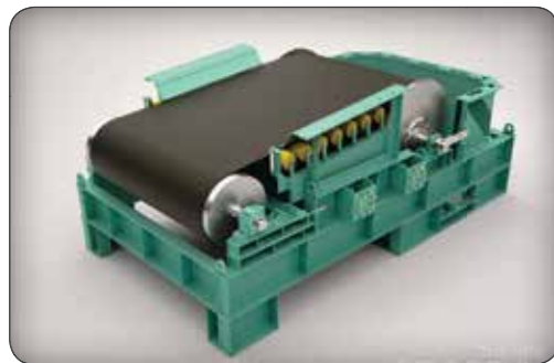
Belt Magnetic Drum Separator
